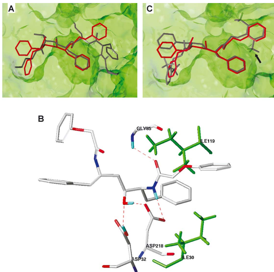
Figure 1. Model structure of TS-98 bound to the active site of C. albicans Sap2. The enzyme structure was based on that of PDB entry 1zap. (A) TS-98 was first docked onto the original inhibitor so as to give a maximum overlap. A-70450 is in grey and TS-98 in red. (B) The original inhibitor was then removed from the active site and the model structure of Sap2 bound to TS-98 minimized and subjected to a molecular dynamics run. H-bonding interactions of TS-98 with enzyme residues, and Ile residues lining a hydrophobic pocket for the Poa group are shown. (C) TS-98 was then replaced by TS-96 and the process repeated; TS-98 is in red, TS-96 is in grey. The region where a methyl group from the P 2 ' dmPoa residue in TS-96 sterically clashes with the active site is indicated by an arrow.
