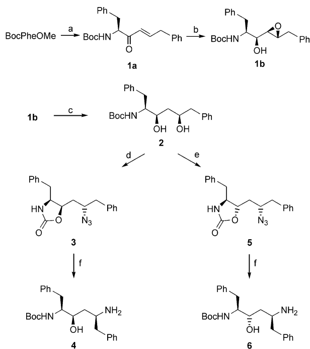
Scheme 2. Synthesis of the diaminoalcohols 4 and 6 , used as central modules in peptidomimetic aspartic protease inhibitors: (a) (i) \text{CH}_3\text{PO}(\text{OCH}_3)_2 , n -BuLi, THF, 95%; (ii) \text{BnCHO} , \text{K}_2\text{CO}_3 , EtOH, 50%; (b) (i) \text{NaBH}_4 , MeOH, 0^\circ\text{C} , 75%; (ii) m CPBA, DCM, 70%; (c) RedAl, THF, 65%; (d) (i) NaH, THF, 80%; (ii) \text{MsCl} , \text{Et}_3\text{N} , DCM; (iii) \text{NaN}_3 , DMSO, 18-crown-6, 80%; (e) (i) 2 equiv \text{MsCl} , DIPEA, 1,2-dichloroethane, 80^\circ\text{C} ; (ii) \text{NaN}_3 , DMSO, 18-crown-6, 50%; (f) (i) \text{Boc}_2\text{O} , NaH, THF; (ii) \text{Cs}_2\text{CO}_3 , MeOH/ \text{H}_2\text{O} ; (iii) \text{H}_2 , Pd/C, 80%.
