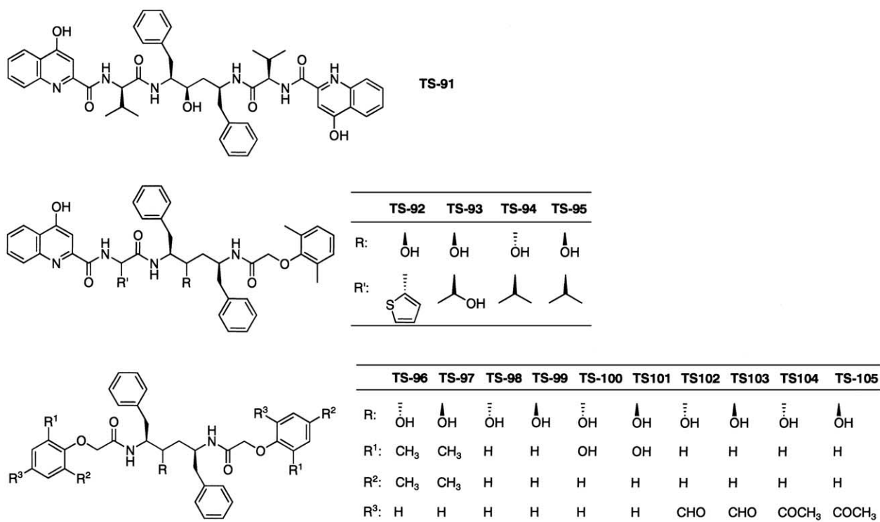
Scheme 3. Structures of peptidomimetic aspartic protease inhibitors reported in Table 1. The stereochemistry of the non-hydrolysable isostere hydroxyl group (R) is indicated.
