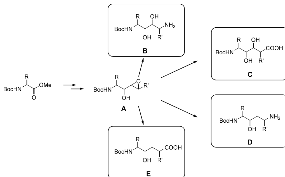
Scheme 1. Overview of dipeptide isosteres available from the common precursor A.
